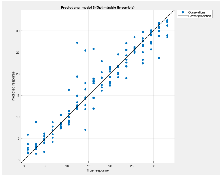
FIGURE 10 ALTITUDE ENSEMBLE OF TREES OPTIMIZABLE CROSS VALIDATION 5 FOLDS PREDICTION PLOT
