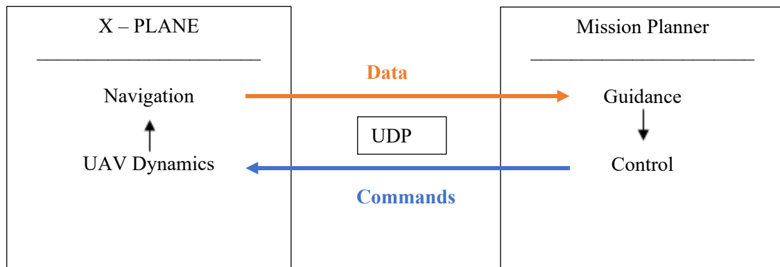
FIGURE 1 X-PLANE – MISSION PLANNER SIL ARCHITECTURE
