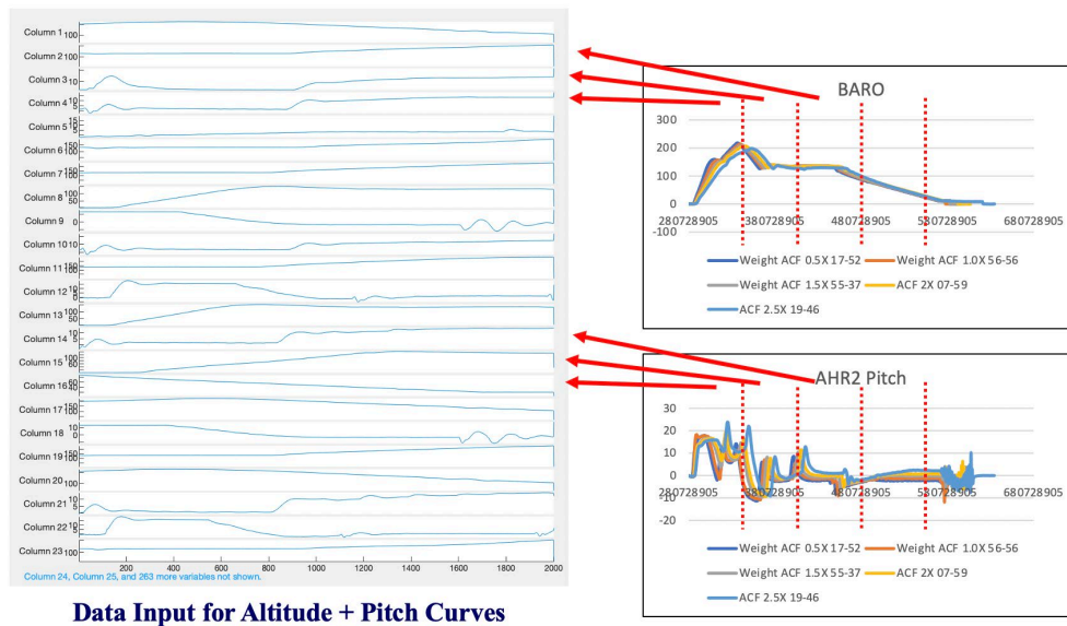
FIGURE 16 ALTITUDE PLUS PITCH INPUT DATA CURVES
