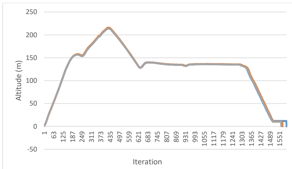
FIGURE 3 ALTITUDE VALUES FOR 3 CONSECUTIVE FLIGHTS FROM THE SAME UAV AFTER REMOVING PRE-TAKE OFF DATA
