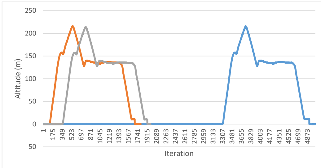
FIGURE 2 ALTITUDE VALUES FOR 3 CONSECUTIVE FLIGHT RUNS OF THE SAME UAV
