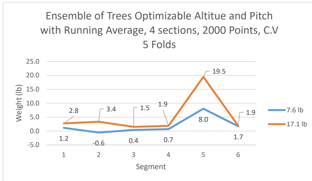
FIGURE 19 ALTITUDE PLUS PITCH ENSEMBLE OF TREES OPTIMIZABLE MODEL CROSS VALIDATION 5 FOLDS RESULTS PLOT
