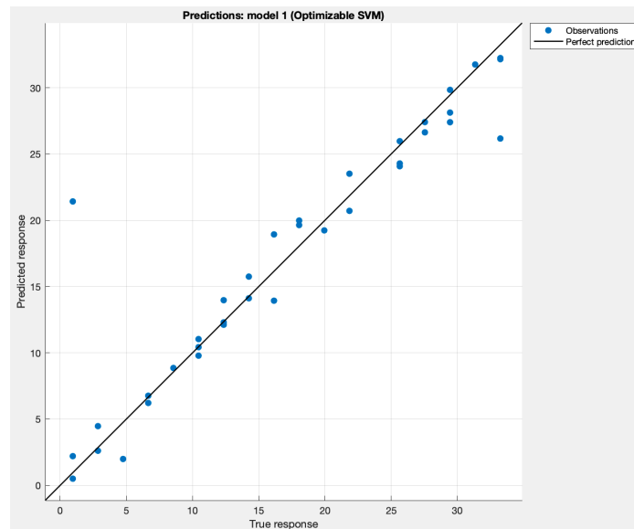
FIGURE 5 ALTITUDE SVM OPTIMIZABLE PREDICTION PLOT
