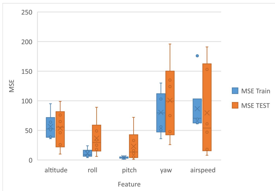
FIGURE 4 SVM REGRESSION ALGORITHM MSE FOR INDIVIDUAL FLIGHT DATA FEATURES
