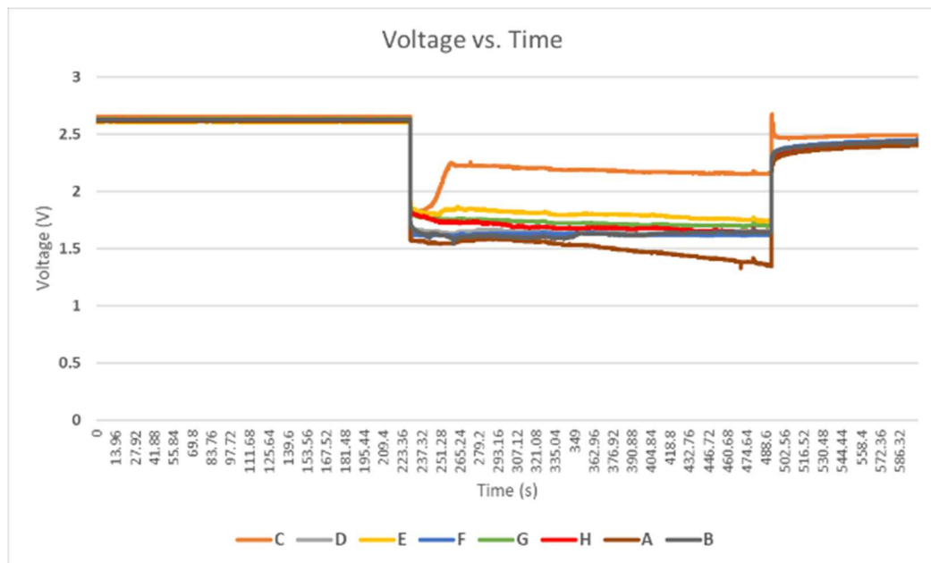
FIGURE 6 REAL-TIME VOLTAGES TOP 2 BATTERIES – EXP. 2, JULY 1
