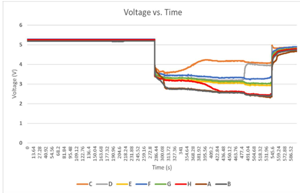
FIGURE 5 REAL-TIME VOLTAGES OF BOTTOM 4 BATTERIES – EXP. 1, JULY 1
