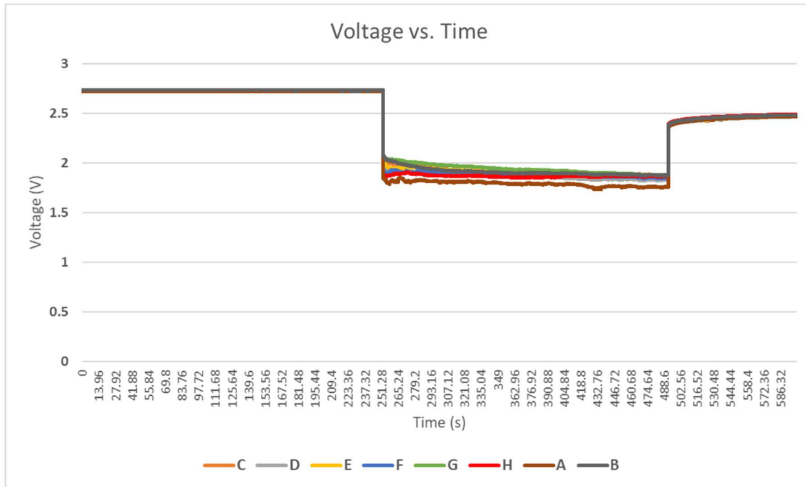
FIGURE 11 REAL-TIME VOLTAGES FOR TOP 2 BATTERIES – EXP. 3, JULY 2
