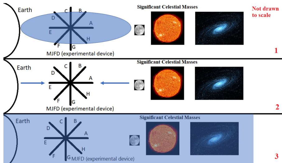
FIGURE 12 VISUAL REPRESENTATIONS OF POSSIBLE NATURES OF THE MACH EFFECT INTERACTION
