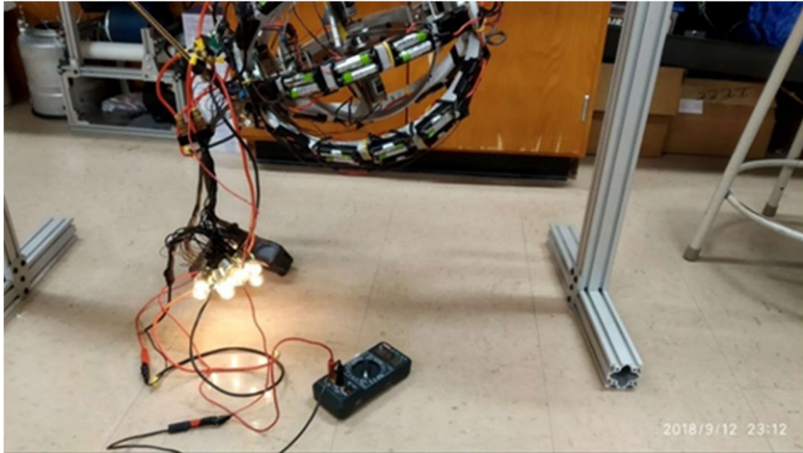
FIGURE 1 MJFD IN LAMP CONTROL EXPERIMENT
