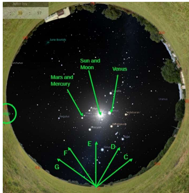
FIGURE 8 STELLARIUM FRONT OF THE EARTH IMAGE FOR EXP. 1, JULY 2 (DAY OF ECLIPSE)
