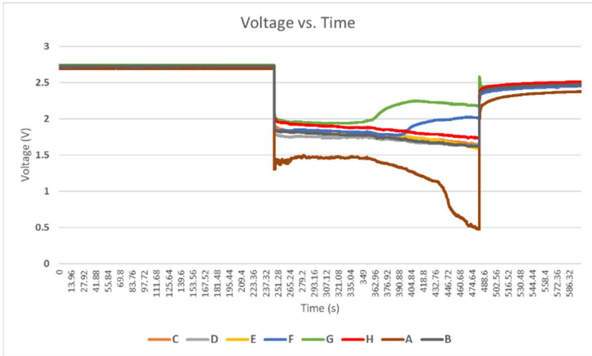
FIGURE 10 REAL-TIME VOLTAGES FOR TOP 2 BATTERIES – EXP. 2, JULY 2
