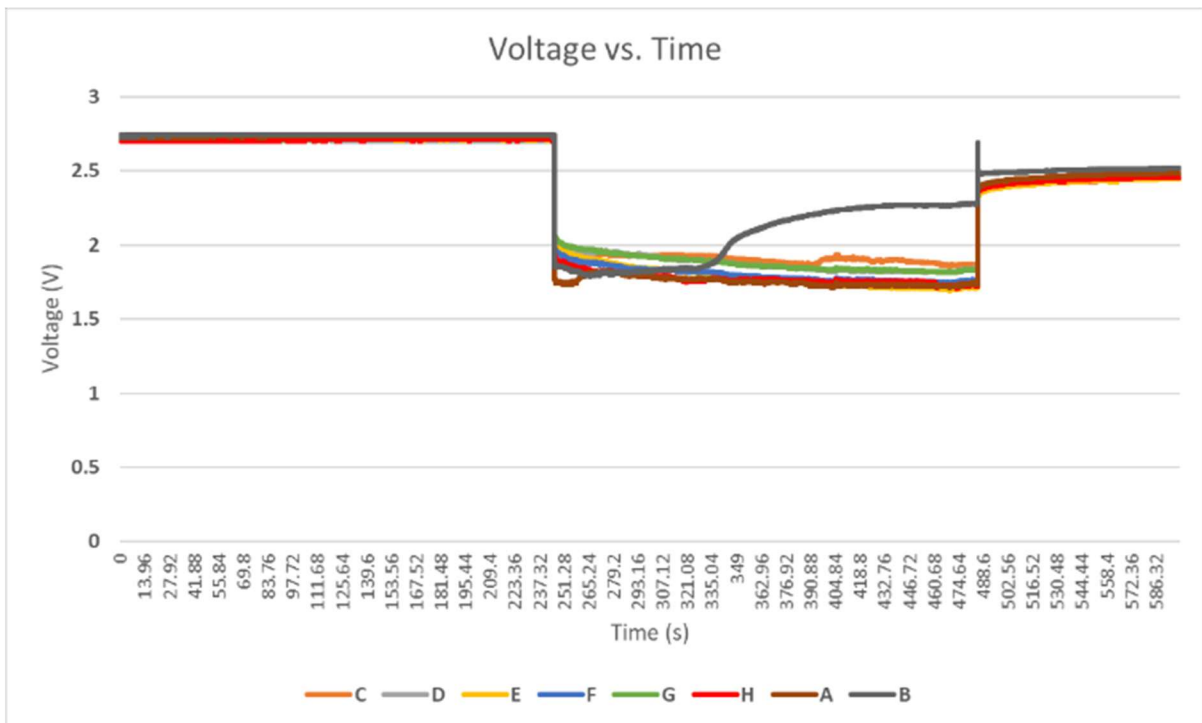
FIGURE 10 REAL-TIME VOLTAGES FOR TOP 2 BATTERIES – EXP. 2, JULY 2
