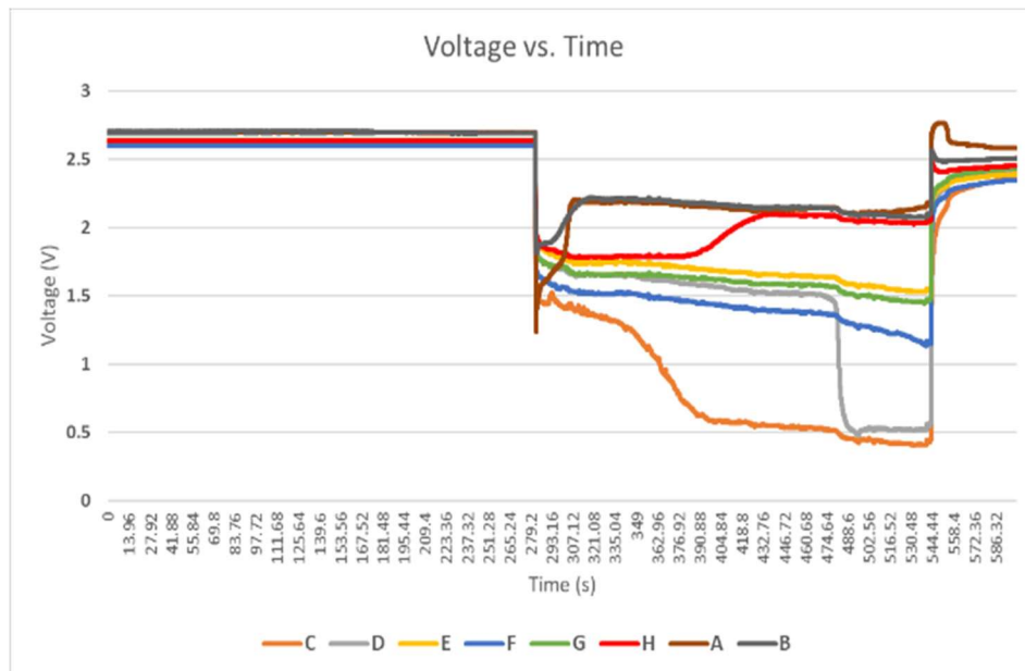
FIGURE 4 REAL-TIME VOLTAGES OF TOP 2 BATTERIES – EXP. 1, JULY 1
