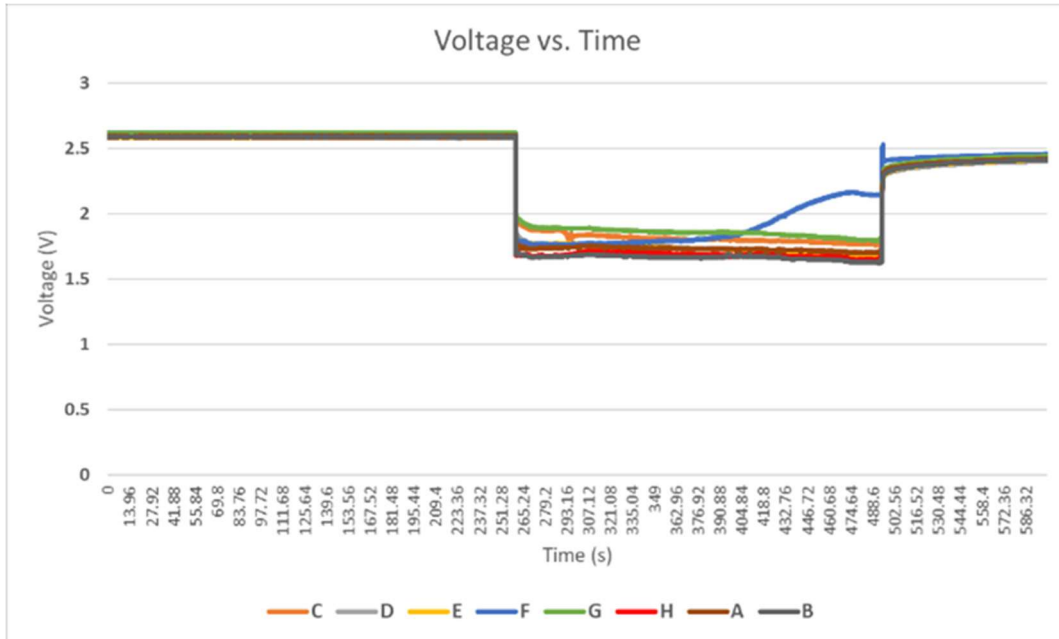
FIGURE 7 REAL-TIME VOLTAGES TOP 2 BATTERIES – EXP. 3, JULY 1
