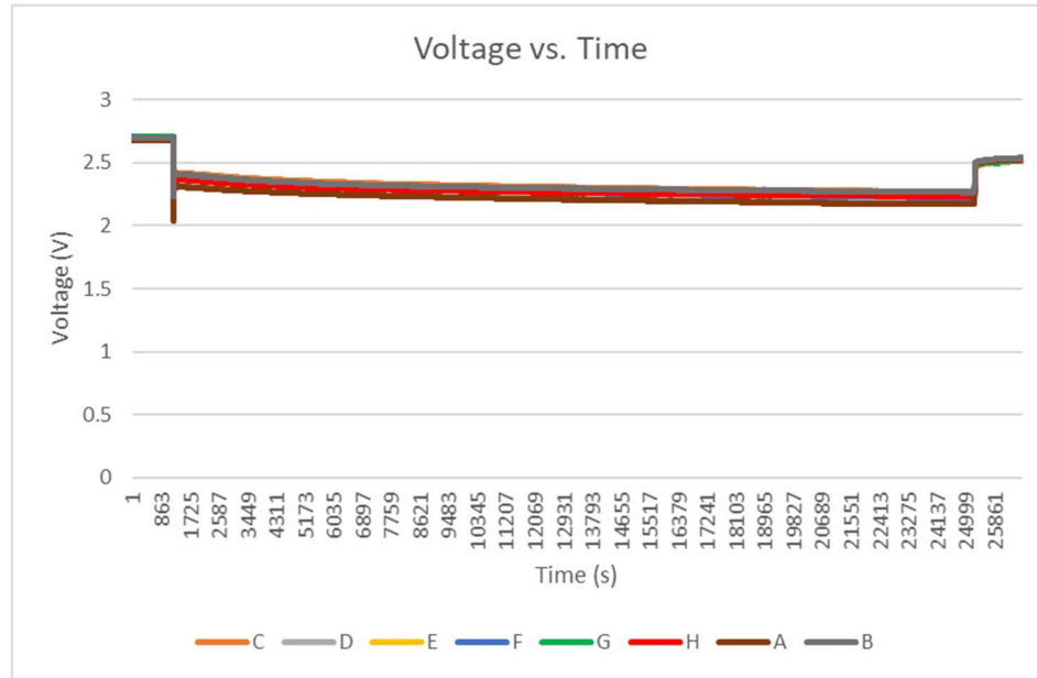
FIGURE 2 TYPICAL DISCHARGE PATTERN FOR BATTERIES IN LAMP CONTROL EXPERIMENT
